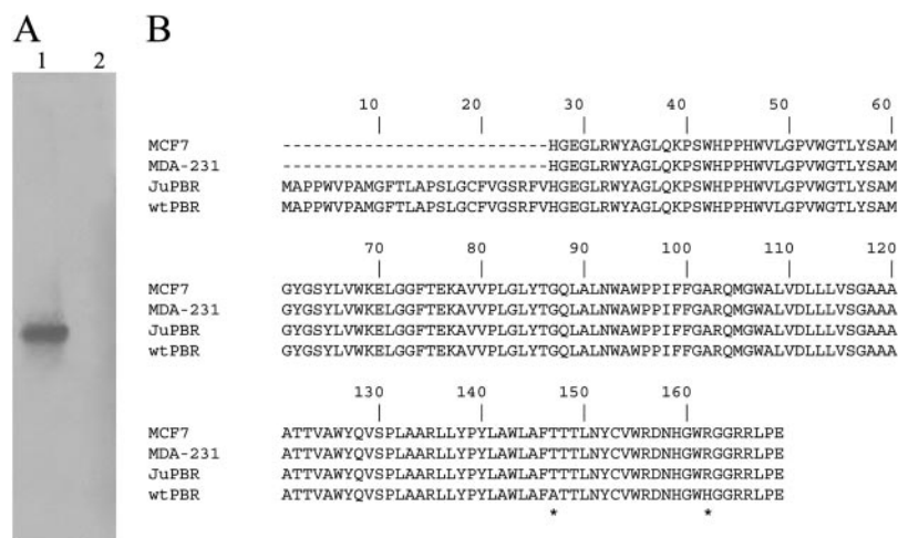
Fig. 1. PBR cDNA isolation in Jurkat cells. A , Southern blot of PBR amplification products. Lane 1, Jurkat cDNA amplified with PBR-specific primers. An autoradiographic band of approximately 600 base pairs was visible. Lane 2, negative RT-PCR control. B , comparison of the deduced amino acid sequence of Jurkat PBR ( JuPBR ) with those of other human PBR protein isoforms: MCF-7, human breast cancer cell line accession number AAC31173.1; MDA-231, human breast cancer cell line (Hardwick et al., 1999); wtPBR, mammalian gene collection program accession number. AAH01110. Asterisks indicate the amino acid substitutions.
